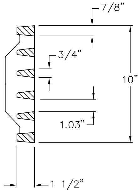
GRATE SECTION
