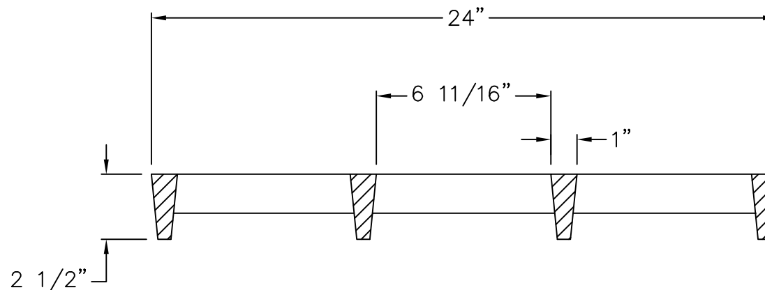
GRATE SECTION
